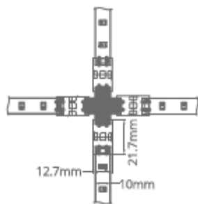
"4" Shaped Connector
