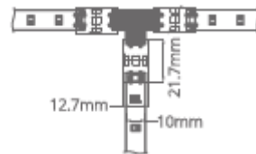
"T" Shaped Connector
